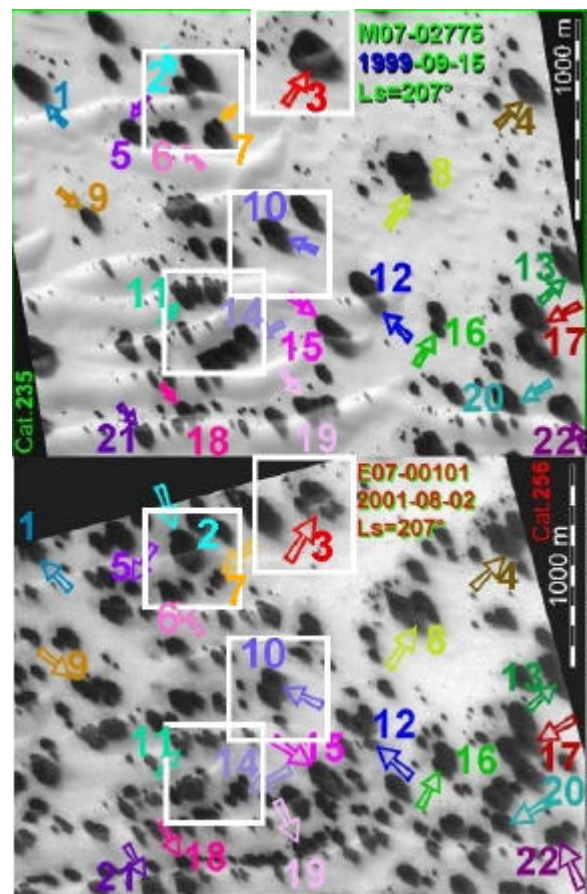
Fig. 2 Reappearing DDSs in the Pityusa Patera, first part of spring 1999 (upper) and 2001 (lower). The numbers with identical color show the identified DDS time-pairs (on identical geographical position). The images shown with white frames can be seen enlarged on Fig. 3.
